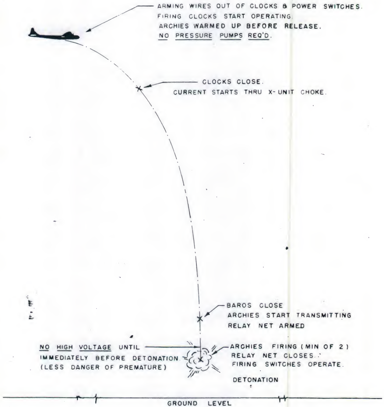
DROP SEQUENCE FOR THE MK IV, MOD 0 ATOMIC BOMB
